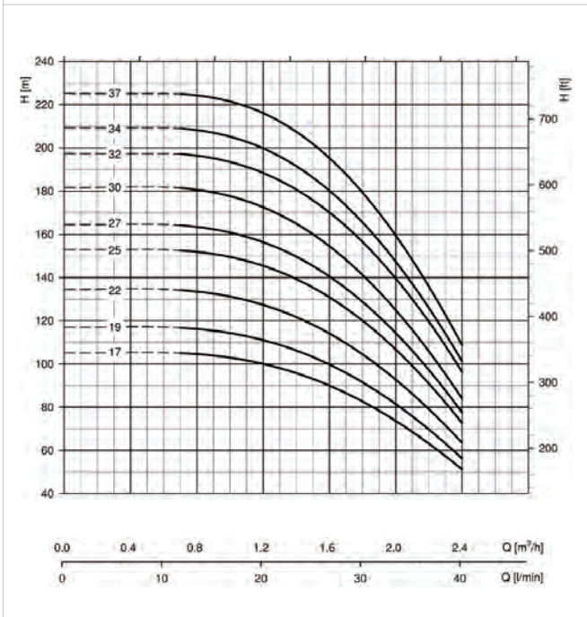
↳ 1SV : 17-37 stages
